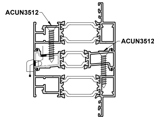
ETC4112
